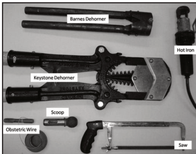
Figure 2. Dehorning Tools
