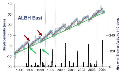
Fig. 4-24. Displacements plotted against time of a GPS station at Albert Head (ALBH), Victoria, B.C., relative to a station at Penticton, B.C., in stable North America. The diagram shows shortening from 1997 through 2004, except for brief periods where the displacement shows lengthening, or extension, of this survey line during episodic tremor and slip. During times of lengthening, seismographs record episodes of seismic tremor, possibly due to movement of fluid on or near the subduction zone. From UNAVCO and Ben Webber based on work by Herb Dragert and Garry Rogers, Pacific Geoscience Centre, Sidney, B.C.
