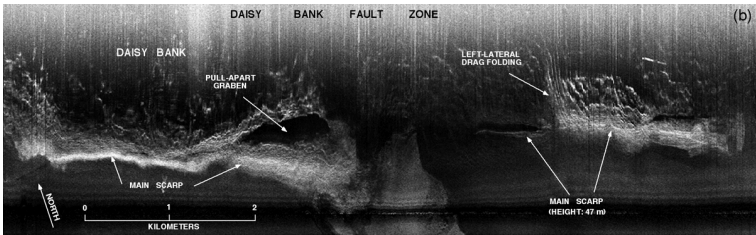
Figure 4-3a. Sidescan sonar image of Daisy Bank strike-slip fault west of Newport. These structures are similar to those on subaerial faults in California. Image from Chris Goldfinger.
