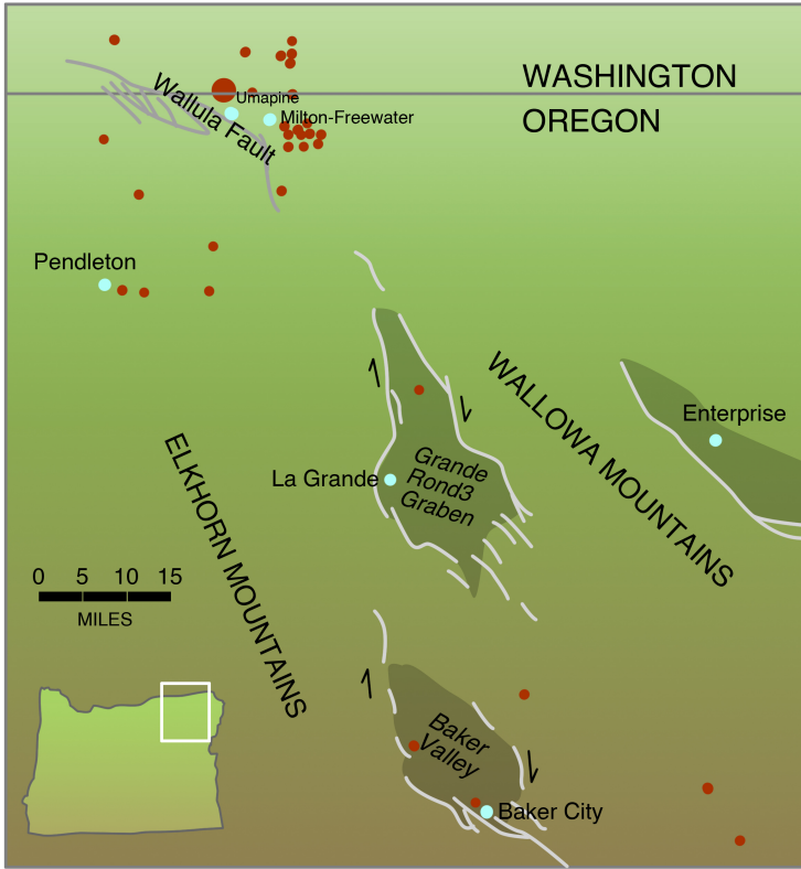
Figure 6-20. Faults in northeastern Oregon in the vicinity of the 1936 Milton-Freewater Earthquake. Shaded areas represent sediment-filled lowlands, including the fault-bounded Grande Ronde Graben and Baker Valley. Solid circles represent earthquakes, with the largest circle the Milton-Freewater Earthquake. This earthquake struck close to the Wallula Fault, but there is no evidence that this fault ruptured the surface during the earthquake. This area is classified as having relatively low seismic hazard by the USGS. Faults and earthquakes from Gary Mann, USGS
