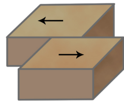
Left Lateral Strike-Slip Fault
