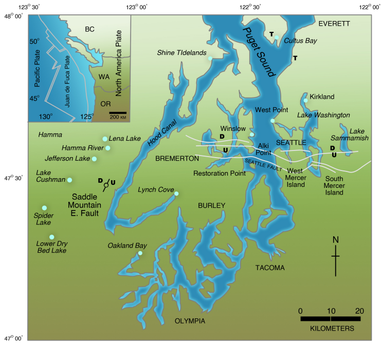
Figure 6-9. The Seattle fault. U means upthrown side, D means downthrown side. Filled upright triangle: uplifted tidal platform; filled upside-down triangle: subsided tidal-marsh deposit; filled circle: tidal-marsh deposit showing no evidence of subsidence; T: tsunami deposit; filled square: rock avalanche; open square: submarine landslide in Lake Washington. Saddle Mt. E. Fault identified as active by J. Wilson and R. Carson. Modified from Robert Bucknam, USGS
