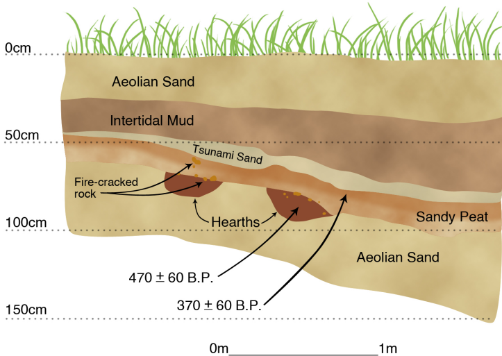
Figure 4-20. Cross section of buried Native American campsite (hearths, fire-cracked rock) overlain by a soil zone submerged by the A.D. 1700 Cascadia Subduction Zone earthquake and covered by a tsunami deposit. From Minor and Grant (1996); drawing courtesy of Rick Minor, Heritage Research Associates, Eugene, Oregon.
