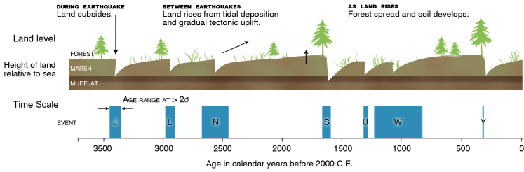
Figure 4-21. Evidence for earthquakes at Redtail locality at Willapa Bay, Washington. Horizontal line is time in years; vertical line is elevation with respect to sea level divided into coastal forest, marsh, and tidal mudflats. Heavy line shows change in elevation. Ground sinks abruptly to sea level after an earthquake, then gradually rises to a marsh environment or a forest environment. Letters identify earthquakes dated by radiocarbon, with the gray band representing uncertainty in dating. The youngest, event Y, is the earthquake of A.D. 1700, dated by tree rings and a tsunami in Japan. The time interval between earthquakes varies from nearly one thousand years between events N and S to less than three hundred years between events U and W. The longest interseismic intervals allowed the ground to develop forests before they were drowned by earthquakes S and Y, whereas earthquakes N, U, and W struck when the ground had only risen to develop a coastal marsh. The greater vertical drop for earthquakes J, S, and Y suggests that they may have been larger than earthquakes N, U, and W. After B. Atwater and E. Hemphill-Haley, USGS
