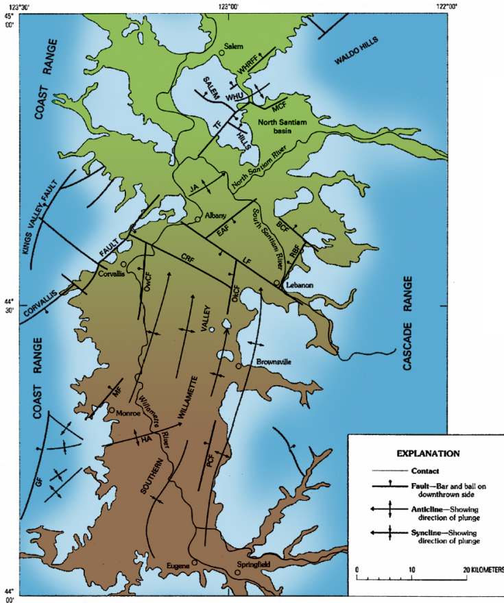
Figure 6-17. Tectonic map of the southern Willamette Valley, using a similar data set to that used for Figure 6-12. From Yeats et al. (1996) and mapping by Erik Graven
