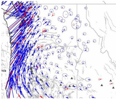
Fig. 3-20. Crustal motion of GPS stations relative to stable North America based on GPS surveys conducted by Pacific Northwest Geodetic Array and Western Canada Geodetic Array. Length of arrow relative to speed of station relative to North America; ellipses at arrow points represent measurement error. Map produced by Rob McCaffrey, Portland State University.
