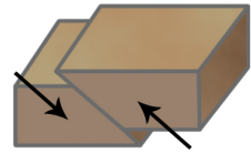
Reverse Fault
