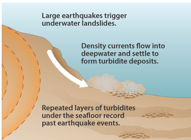
Figure 4-6. Diagrammatic representation of Cascadia turbidite sand avalanche triggered by a subduction-zone earthquake. Figure prepared by Kathleen Cantner, American Geosciences Institute, used with permission.
