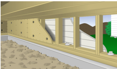
Figure 11-3. Cripple wall between the foundation and house. Wall is bolted to foundation. Plywood contains air holes to disperse moisture.
