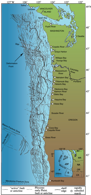
Figure 4-12. The Pacific Northwest coast locating sites of coseismic subsidence on the coast from Vancouver Island to northern California (open circles). From Sixes River to Vancouver Island, subsidence is due to subduction-zone earthquake. Subsidence at Humboldt Bay is related to crustal faulting (see Chapter 6). Active offshore faults and folds are also shown. Heavy line is the edge of the continental shelf. Image courtesy of Lisa
