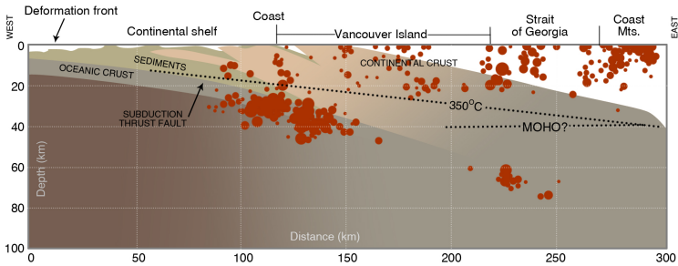
Figure 5-9. Cross section of the Cascadia Subduction Zone across southern Vancouver Island showing crustal structure based on surface geology, a deep seismic-reflection profile, the distribution of earthquakes located by seismographs (filled dots; size proportional to magnitude), and temperature based on geothermal measurements onshore and offshore. From Garry Rogers and Roy Hyndman, Pacific Geoscience Centre, Sidney, B.C.
