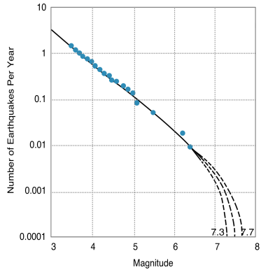
Figure 7-4. Gutenberg-Richter curve for crustal earthquakes in the Puget Sound and southern Georgia Strait region. The data are reliable for earthquakes of M 3.5 to 5 and less reliable for earthquakes of M about 6.2. The curve indicates 0.1 earthquake of M 5 per year, which is the same as one earthquake per ten years. An earthquake of M 6 would be expected every fifty years. The curve is not extended as a straight line to higher magnitudes, but instead is curved downward to approach a vertical line, which would be the maximum earthquake expected in the region (a deterministic estimate), estimated as M 7.3 to 7.7. From Roy Hyndman and Kelin Wang, Pacific Geoscience Centre
