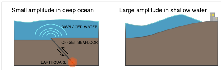
Figure 9-7. (Left) Formation of a tsunami by sudden offset of the sea floor. Wave has a low amplitude as it travels in the deep sea. (Right) Wave amplitude grows as tsunami enters shallow water and approaches the land.
