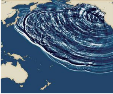
Figure 4-18. Computer model of Cascadia subduction-zone earthquake, from Kenji Satake and his colleagues at the University of Tokyo.
