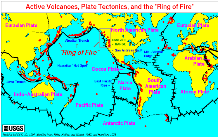
Figure 2-3b. Earth's surface divided into tectonic plates. Thickest boundaries: subduction zones; thinner lines: spreading centers. Red dots locate active volcanoes, largest adjacent to subduction zones. Note location of Ring of Fire, of which Cascadia (open rectangle) is a part.
