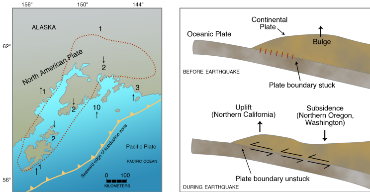
Figure 4-14. (Right) Cross section showing buildup of elastic strain in North American continental edge before an earthquake, then sudden release (elastic rebound) during earthquake, causing the outermost part of upper plate to go up and an inner part to go down. The Vancouver Island, Washington, and Oregon coast should go down and the northern California coast should go up, according to this model. Modified from Brian Atwater, U.SGS. (Left) Map of part of southern Alaska, showing parts of the crust that went down in the great 1964 earthquake (Mw 9.2) and parts that went up. Numbers show subsidence (down arrows) or uplift (up arrows) in meters. Uplift and subsidence accompanying this earthquake were used to model uplift and subsidence accompanying a Cascadia Subduction Zone earthquake. Images courtesy of Chris Goldfinger, College of Earth, Ocean, and Atmospheric Sciences, OSU.
