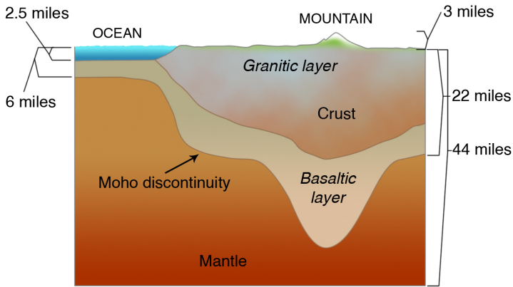
Figure 2-2. Cross section of oceanic crust (left) and continental crust (center and right). Continent is composed of granitic rock which is lighter, thicker, and more buoyant than oceanic crust, which is underlain by heavier basaltic rock. Both continental and oceanic crust overlie the mantle, composed of peridotite. The top of the mantle is the Moho. The continent stands high with respect to the ocean basin, and for it to be in balance, it's underlain by a deep root of lighter crust. Mountain ranges stand above the continent and are underlain by still deeper roots. From Yeats et al. (1997), with permission
