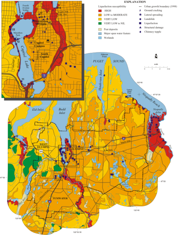
Figure 8-16. Liquefaction susceptibility map of the Olympia-Tumwater-Lacey area, Washington, published as Washington Division of Geology and Earth Resources GM-47 (Palmer et al., 1999). The darkest shading identifies those areas most susceptible to liquefaction and lateral spreading. The damage from liquefaction and lateral spreading from the 2001 Nisqually Earthquake is superimposed on this map, showing how well the map predicted the zones of damage, especially in downtown Olympia. From Tim Walsh, Washington Division of
