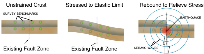
Figure 3-3. Illustration of elastic rebound theory of Harry F. Reid. Strain is building up.
