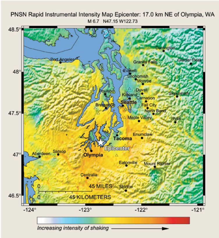
Figure 3-17. Experimental ShakeMap for Nisqually Earthquake based on forty-nine strong-motion seismograms (triangles), sixteen of which recorded peak accelerations greater than 10 percent g and two greater than 25 percent g . Map takes into account ground conditions and is generated automatically. Darker areas around epicenter (filled star) have accelerations greater than 9.2 percent g . Accelerations greater than 18 percent g are found in a linear band extending from Seattle toward Eatonville and patches south of Olympia and west of Interstate 5 as well as east of Olympia. The lighter patch in and southwest of Tacoma represents accelerations lower than 9 percent g . The objective of ShakeMap is to locate areas quickly enough to direct emergency services to the areas of strongest shaking. From the Pacific Northwest Seismograph Network.
