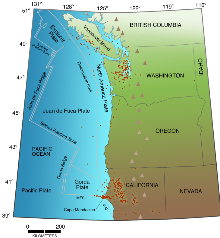
Figure 5-1. Distribution of earthquakes deeper than 16 miles in the Pacific Northwest. Most are intraplate earthquakes in the downgoing Juan de Fuca Plate. Earthquakes are not distributed evenly but are concentrated in Puget Sound, coastal Vancouver Island, and northwestern California. MFS, Mendocino Fracture System; SAF, San Andreas Fault; Heavy curved line in western Washington locates the top of the subduction zone at 60 km depth. Triangles: Cascade volcanoes. (100 km = 62 miles). From USGS Professional Paper 1560.
