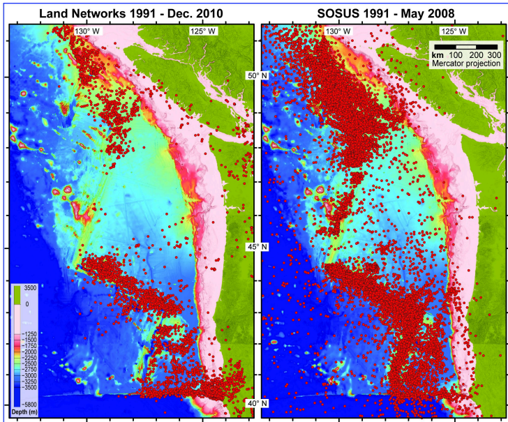
Fig. 4-13. Seismicity of the offshore Pacific Northwest and Vancouver Island based on land networks of seismographs (left) and a highly-sensitive hydrophone array (Sound Surveillance System, or SOSUS) that transmits sound through the water column (right). Even at this sensitivity, the Cascadia Subduction Zone is not generating earthquakes in the region between southern Vancouver Island and northern California. The large number of earthquake off northern Vancouver Island are on the Explorer Plate; much of the Gorda Plate is seismically active due to internal deformation. But not the subduction zone. From Bob Dziak, NOAA and OSU.
