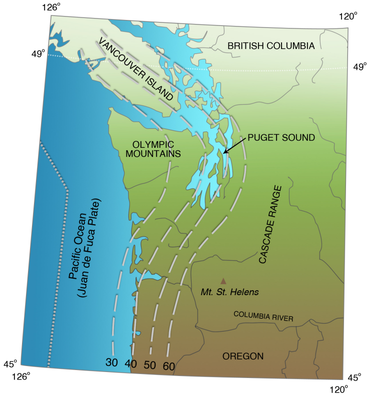
Figure 5-8. The distribution of slab earthquakes helps determine the contours of the top of the Juan de Fuca Plate, in kilometers below sea level. Notice that these contours are convex to the east, causing compression within the slab as it subducts beneath North America, analogous to the folds in a tablecloth at the corner of a table. From Robert Crosson, University of Washington
