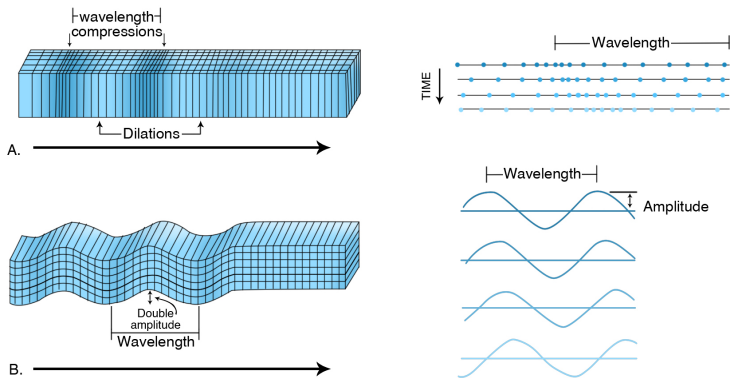
Figure 3-12. Two views of (a) P waves and (b) S waves, all moving from left to right. A P wave moves by alternately compressing and dilating the material through which it passes, somewhat analogous to stop-and-go traffic on the freeway during rush hour. An S wave moves by shearing the material from side to side, analogous to flipping a rope tied to a tree. Note the illustration of wavelength for P and S waves and amplitude for S waves. The number of complete wavelengths to pass a point in a second is the frequency. Low-frequency body waves of large earthquakes travel on a curving path through the Earth for thousands of miles to reach seismographs around the world (Figure 3-11). I pointed out earlier that only the outermost parts of the Earth are elastic. How can the mantle, which is capable of the slow plastic flow that drives plate tectonics, also behave as an elastic solid when earthquake body waves pass through it?
