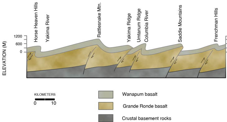
Figure 6-23. Geologic cross section across Yakima Fold Belt west of Hanford Reservation. Folds in basalt are interpreted as being forced up by compressional faults in rigid crust beneath the basalt; these faults may be earthquake sources. South is to the left.
