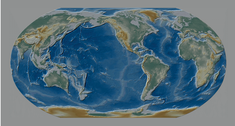
Figure 2-3a. World map with oceans removed. Ocean floor in shades of blue; lightest bands show oceanic spreading centers (Mid-Atlantic Ridge, East Pacific Rise) and very dark bands show trenches, the boundaries of subduction zones. Light band at west edge of North America locates continental slope, at base of which is Cascadia Subduction Zone.
