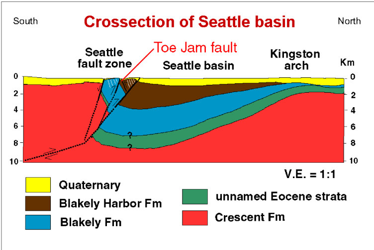
Fig. 6-10. Cross section of Seattle fault, showing that the north side is downdropped as part of the Seattle basin, and the south side is uplifted, with bedrock close to the surface. This is evidence that the deformation around 1100 years ago was part of long-term deformation of the Seattle region.
