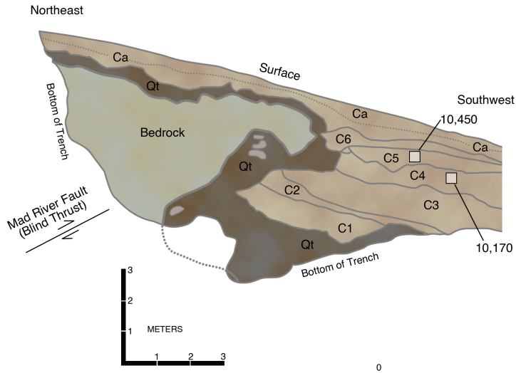
Figure 6-36. Log of side of backhoe trench across a scarp of the Mad River Thrust Fault at McKinleyville, California, showing how bedrock has been thrust over sediments that are radiocarbon dated at about ten thousand years. Laboratory errors are \pm 60\text{--}80 years. The bedrock is overlain by a wave-cut platform which is itself overlain by terrace deposits (Qt). These were folded, indicating that the Mad River Fault is a blind thrust at this locality. The terrace deposits are overlain by debris from the rising fault scarp (C1 through C6); each unit may have been deposited during an earthquake. Ca marks the active slope wash and debris. Modified from a sketch by Gary Carver, Humboldt State University
