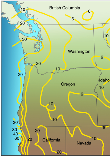
Figure 8-3. Map of the Pacific Northwest showing earthquake horizontal accelerations having a 10 percent probability of being exceeded in fifty years for a firm rock site (Soil Class B site in Canada). Contours in percent gravity (g). From USGS and Geological Survey of Canada (Basham et al., 1997). USGS map revised in 2002
