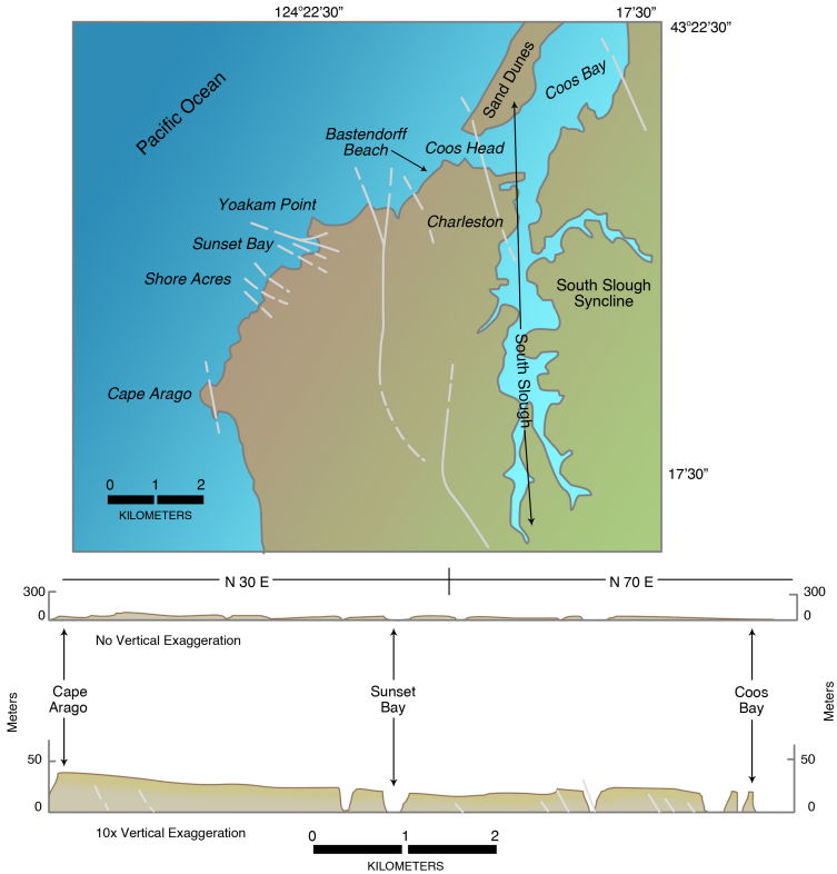
Figure 6-33. (Top) Map of Cape Arago-Coos Bay region, southwest Oregon, showing marine terrace platforms and active faults. (Bottom) Cross section along the coast from Cape Arago to Coos Bay showing tilting and faulting of Whiskey Run marine terrace and platform, eighty thousand years old. One cross section shows the vertical scale exaggerated ten times the horizontal scale, the other shows the cross section without vertical exaggeration. From G. McNelly and H. Kelsey, Humboldt State University
