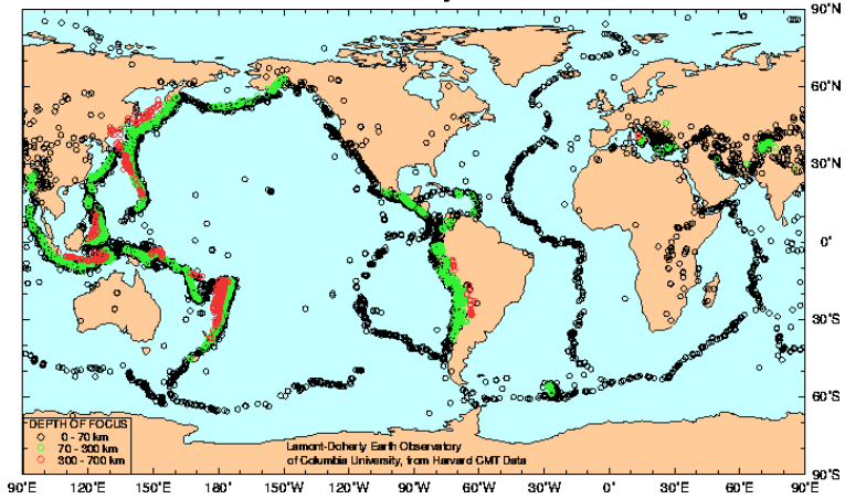
Figure 2-5. World map of seismicity, showing larger earthquakes. Most (but not all) earthquakes follow plate boundaries. Colors adjacent to subduction zones show earthquake focal depths: green for depths 70-300 kilometers, red for deeper earthquakes to 700 km. No color indicates earthquakes shallower than 70 km.
