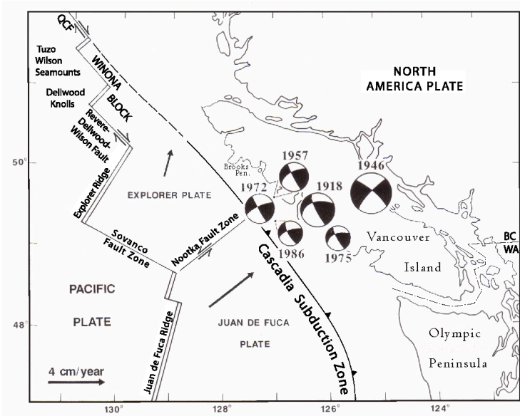
Figure 6-19. Earthquakes northeast of Nootka fault zone and central Vancouver Island. The Nootka fault zone separates the Juan de Fuca and Explorer plates. The beach-ball plots show that all earthquakes were due to left-lateral strike slip; larger earthquakes have larger beach balls. The 1918 and 1946 earthquakes were in North American continental crust. The 1946 earthquake was the largest recorded crustal earthquake in the Cascadia region. QCF: Queen Charlotte fault.
