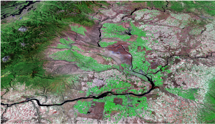
Fig. 6-22. Oblique digital image of Yakima fold belt, view north. Image courtesy of William Bowen, California State University Northridge and California Geographical Survey. Columbia River doubles back on itself at Wallula Gap and flows west toward Portland. Linear features are Yakima folds. Farther west are three Cascade volcanoes and in upper left corner, the waters of Puget Sound. Compare with top map of Figure 6-21, which identifies major Yakima folds.
