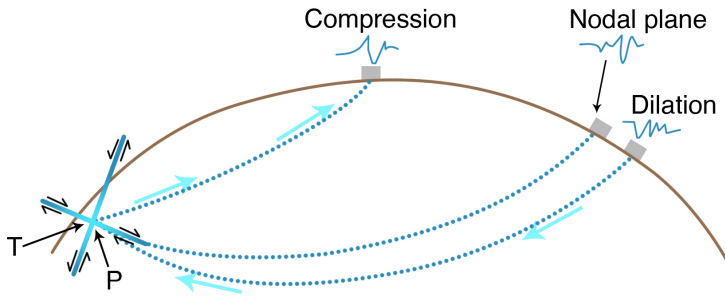
Figure 3-18. Use of first motion of seismic wave at several seismographs (open boxes) to determine mode of earthquake faulting. One seismogram shows a compression (first wave goes up, reading from left to right), indicating that the first motion was away from the source. Another shows a dilation (first wave goes down), indicating that the first motion was toward the source. A third is indeterminate, suggesting that it is on the boundary between compression and dilation. From this, we can determine that the earthquake was on a normal fault, even though we don't know which of the two planes is the true fault plane. Lines are curved because of different speeds of seismic waves in the Earth. Modified from Yeats et al. (1997), with permission of Oxford University Press.
