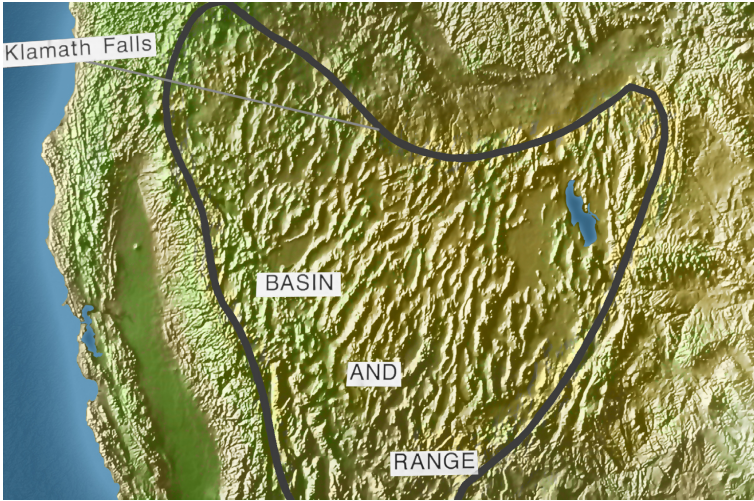
Figure 6-31. A Computer-generated topographic map of the Basin and Range Province. The linear pattern is formed by block-fault mountain ranges bound by normal faults and separated by valleys and grabens. From USGS.
