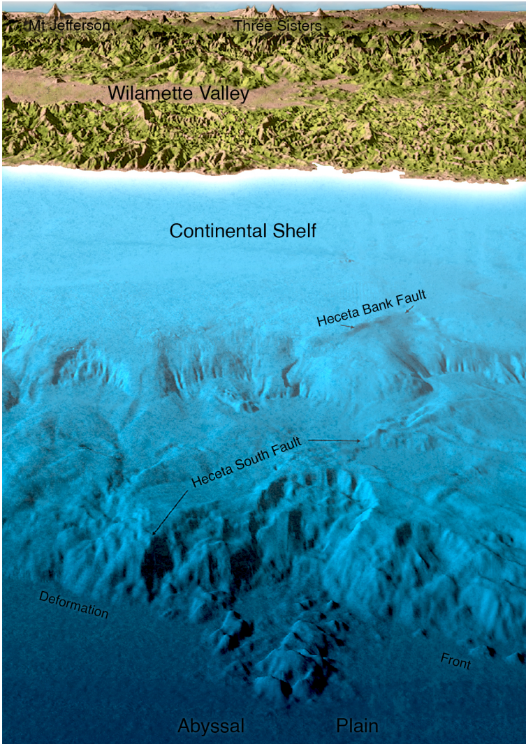
Figure 8-14. Large landslide at the base of the continental slope west of Florence, Oregon. Slide is five miles across; debris has been transported across the deformation front onto the Juan de Fuca abyssal plain. The active Heceta South Fault marks part of the northern side of the slide. Image created by Chris Goldfinger at Oregon State University from SeaBeam bathymetric maps of the National Oceanic and Atmospheric Agency and digitized
