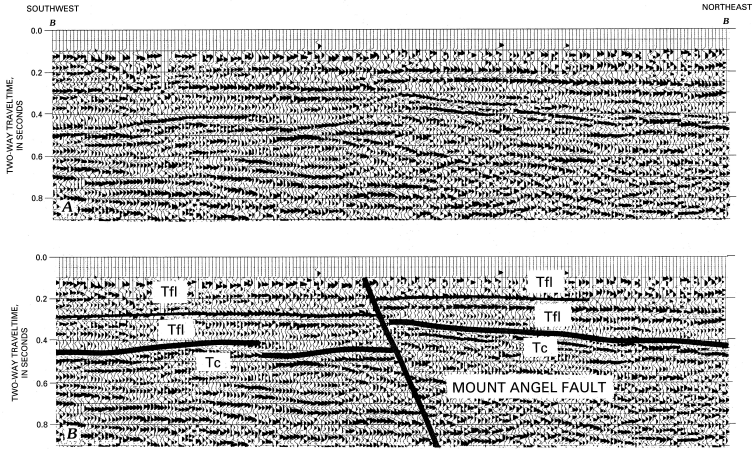
Figure 6-18. Seismic-reflection profile obtained in the search for oil and gas in the Willamette Valley. The horizontal lines are layers of rock beneath the surface that have been offset by the Mount Angel Fault. The bottom diagram is identical to the top one except it contains a geologic interpretation. Tc = Columbia River Basalt; Ttl = younger sediment filling the northern Willamette Valley. Photo by Ken Werner, Oregon State University, from Yeats et al. (1996)
