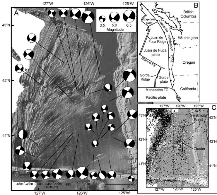
Figure 2-4. A sonar image of Gorda Plate, in which lines represent former positions of the Gorda Ridge spreading center, the current location of which is at the lower left. At bottom, east-west ridge is Mendocino Fracture Zone (FZ) between Gorda and Pacific plates. At upper left is Blanco Fracture Zone. Cascadia Subduction Zone is at far right, between Gorda Plate and North American Plate. Circles (beach balls) represent fault-plane solutions, described in Chapter 3; see Fig. 3-19. B. Plate tectonic map of Cascadia. C. Dots locate microearthquakes measured by seismographs and hydrophone arrays.
