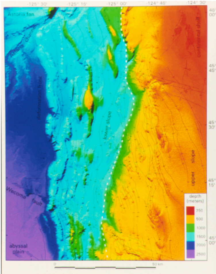
Figure 4-4. Computer-generated sea-floor image of the Oregon continental slope west of Seaside and Cannon Beach, based on sea floor topographic mapping by the National Oceanic and Atmospheric Administration. Elongate hills are anticlines formed by folding of sediment when plates collided at the Cascadia Subduction Zone (marked “deformation front”). The seaward end of the Astoria Submarine Canyon and Channel is seen at upper left. Canyons such as this contain turbidity-current deposits triggered by subduction-zone earthquakes. Image courtesy of Chris Goldfinger, College of Earth, Ocean and Atmospheric Sciences, Oregon State
