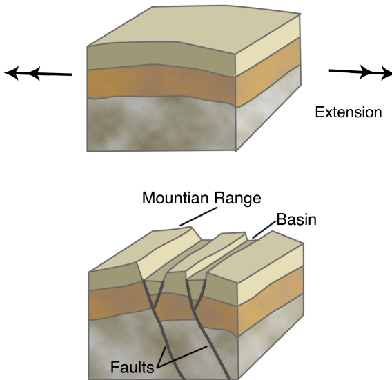
Figure 6-27. Structure of the Basin and Range Province of southeastern Oregon. Because the crust is extending east-west, normal faults form. The basin formed between two opposing normal faults is called a graben. Upper Klamath Lake (Figure 6-20) occupies a graben.
