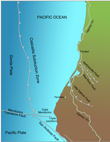
Figure 4-22. Computer-generated topographic map of California north coast showing the Triple Junction, the San Andreas Fault, the Mendocino Transform Fault, the Cascadia Subduction Zone, and active thrust faults onshore.
