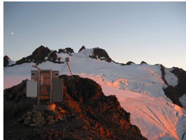
Figure 3-19. Global Positioning System (GPS) survey, part of the Pacific Northwest Geodetic Array (PANGA), of a rock outcrop on the Snow Dome on the north side of Mount Olympus, Olympic National Park. Photo by Spencer Reeder, Central Washington University
