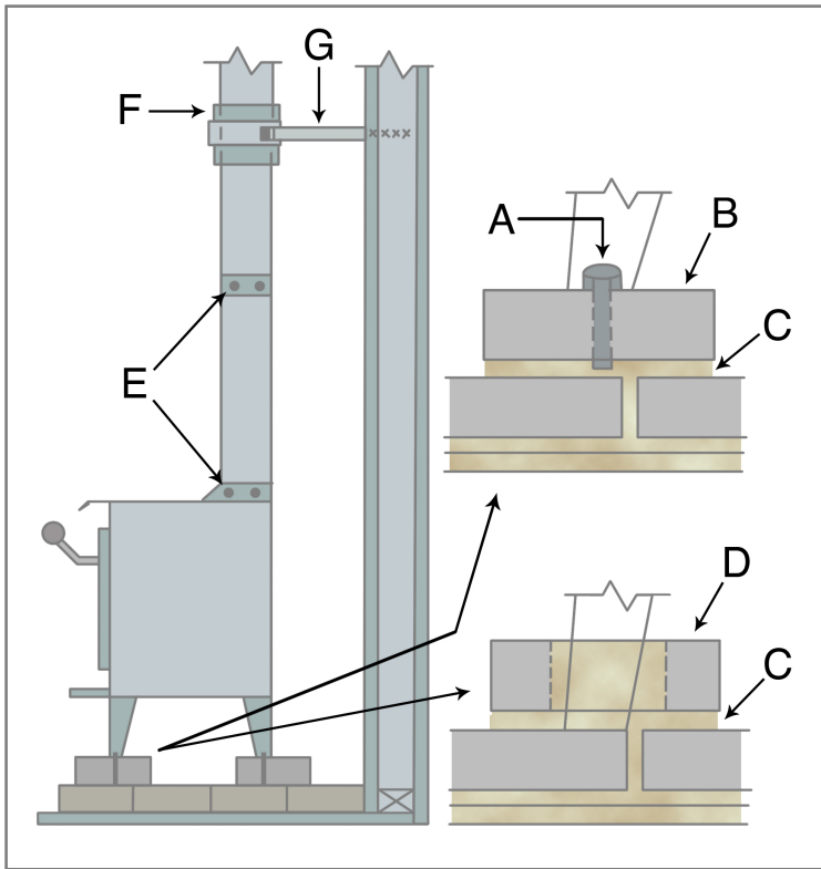
Figure 11-14. Anchor a stove built on a brick hearth with three-eighths-inch diameter bolt (A) through half-inch hole to new brick (B). Grout brick to existing hearth with one inch of new grout (C). As an alternative, build an eight-inch-square brick pad with grout pocket (D) at each leg. There should be at least one inch of grout around each leg; fill pocket completely with grout. Provide sheet metal screws (E) at flue exit and between stovepipe sections. Provide a radiation shield with pipe clamp (F) braced to wall, using tension ties attached to wall stud with three-eighths-inch by three-inch lag screws. From Humboldt Earthquake Education Center, Humboldt State University
