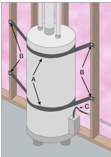
Figure 11-8. Strap water heater, top and bottom, with metal straps (A) which completely encircle the heater and are attached to studs (B). If the water is heated by gas, the gas supply line (C) should be flexible. In this example, water heater rests against stud. If water heater is against drywall or plaster wall, brace it with a two-by-four so that it does not bang against the wall.
