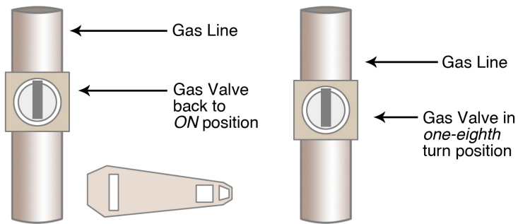
Figure 11-7. Shut-off valve for the main gas supply line to house. Left: valve in "on" position. Right: Check to be sure valve is not frozen by turning it one-eighth turn. Specialized wrench available from gas company is also shown.
