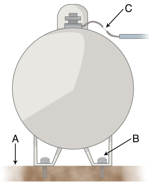
Figure 11-15. Propane tank. Mount tank on six-inch-thick concrete pad (A) using four half-inch diameter bolts (B) with three-inch minimum embedded into concrete. Provide a flexible hose connection (C) between tank and the rigid supply line. From Humboldt State University
