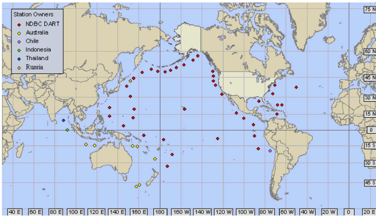
Fig. 9-12. Distribution of DART buoys in Pacific Ocean at time of Tohoku-oki Earthquake in northeast Japan.
