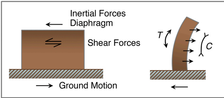
Figure 12-5. Shear walls resist shear stresses transmitted from the ground and bending stresses in slender, tall buildings. C, compression; T, tension. From AIA/ACSA Council on Architectural Research.
