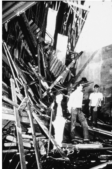
Figure 5-3. Puyallup High School damaged in 1949 earthquake. Unanchored roof and ceiling beams over the stage of the auditorium slid off supporting walls and crashed to the floor. From Thorsen (1986); illustration from collection of Washington Division of Geology and Earth Resources
