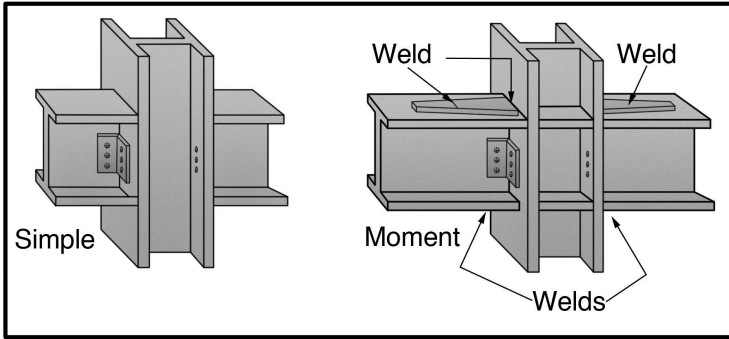
Figure 12-6. Joint used in a moment-resistant frame.
