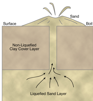
Figure 8-5. Vertical cross section through a sand boil, showing the liquefied sand layer, nonliquefiable clay cap, and the sand dike transmitting the liquefied sand to the surface, forming a sand boil or sand volcano. From Steve Obermeier, USGS
