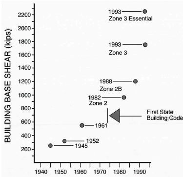
Figure 14-2. Change in building codes in Oregon since 1945 for a typical mid-rise building with respect to seismic base shear force (horizontal) measured in kips (1 kip = 1,000 pounds per square inch). With this diagram and the age of the building, it can be determined how much shear resistance was allowable in the building when it was constructed. From Grant Davis, KPFF Consulting Engineers, courtesy of Franz Rad, Portland State University
