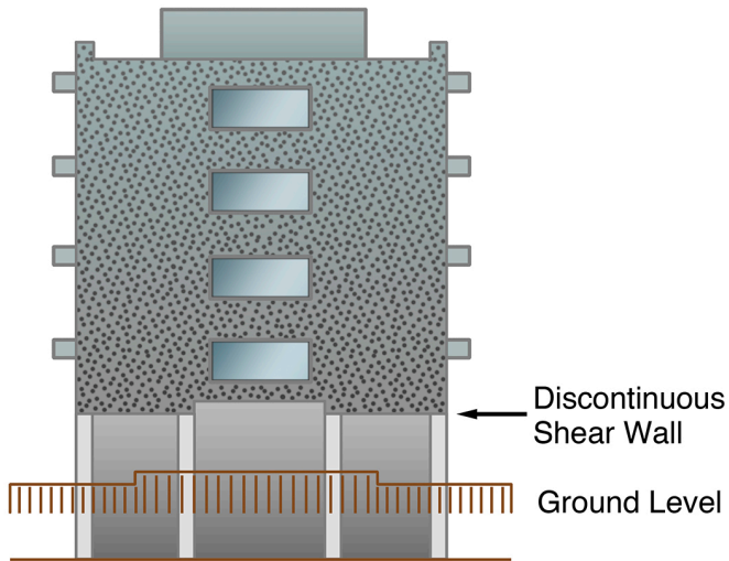
Figure 12-11. Diagrammatic representation of soft story at Olive View Medical Center. From AIA/ACSA Council on Architectural Research
