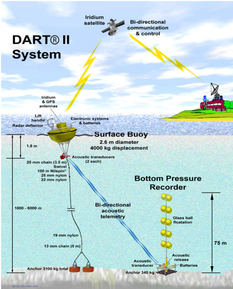
Fig. 9-11. A DART buoy installed by NOAA as part of a tsunami warning service. The buoy is connected to a pressure recorder on the sea bottom that transmits the elevated pressure of a tsunami wave passing over it. This information is transmitted to the two tsunami warning centers in Hawaii and Alaska.
