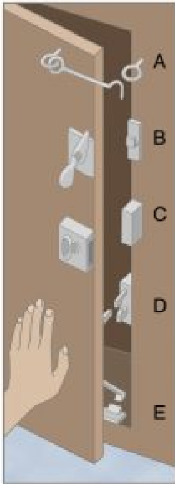
Figure 11-11. Safety latches for earthquakes. The simple hook and eye (A) is inexpensive and secure, but you may not remember to close it each time you use the cabinet because it takes an extra step to do so. Some latches (B, C) mount on
