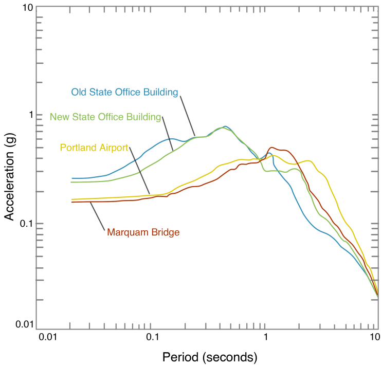
Figure 8-2. Acceleration, in percent gravity (g) of seismic waves of different periods from a postulated Cascadia Subduction Zone earthquake at four soil sites in Portland. Earthquake is 120 km from Portland. From Wong et al. (1993)
