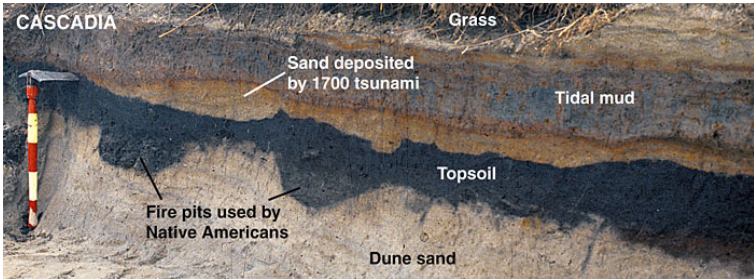
Figure 9-5b. Photo of 1700 tsunami overlying topsoil and Native American fire pits at Salmon River, Oregon.
