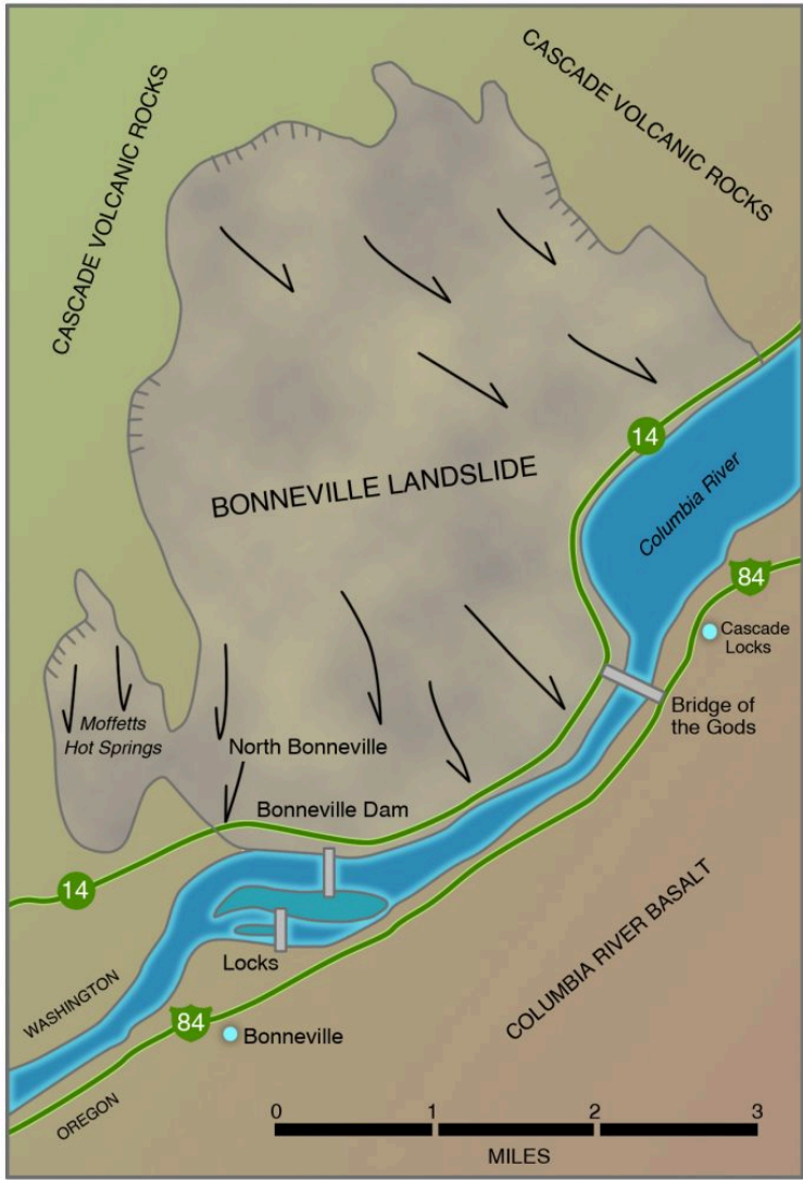
Figure 8-15. Map of the Bonneville landslide (shaded) in the Columbia River Gorge at Cascade Locks. Arrows show direction of flow of landslide material. Bedrock formations shown in clear pattern. Volcanic rocks of the Cascade Range underlie the slide on the Washington side of the Columbia River; Columbia River Basalt is found on the Oregon side. Based on work by Bob
