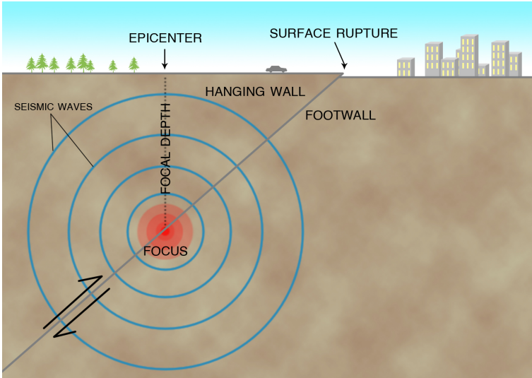
Figure 3-4. A cross section of the Earth's crust.
