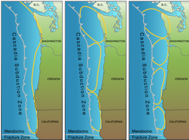
Figure 7-2. The deterministic choices for the maximum considered earthquake on the Cascadia Subduction Zone. (Left) The entire subduction zone ruptures at the same time, resulting in an earthquake of MW 9+. (Center and right) Segments of the subduction zone of various sizes rupture independently, resulting in smaller earthquakes. Modified from Alan Nelson and Stephen Personius, USGS
