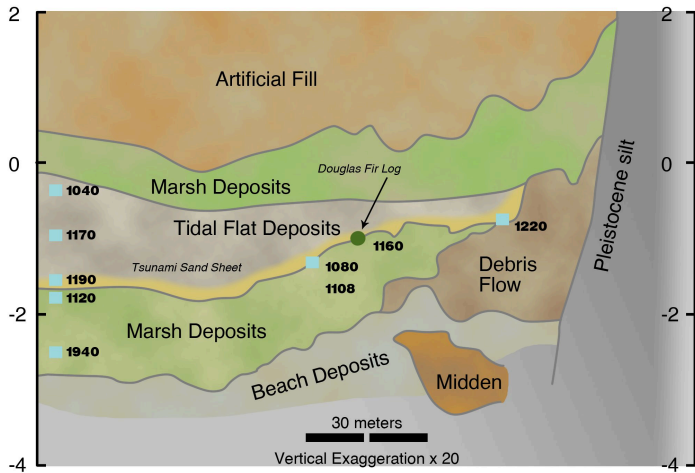
Figure 6-6b. Log of walls of excavation for sewer line. Shaded squares locate samples for radiocarbon dates, which are given in radiocarbon years before 1950 A.D., with laboratory error bars \pm 50 to 80 years. Beach deposits at least two thousand years old contain a midden where people had built fires and thrown away shells. This is overlain by a marsh deposit containing marsh grass stems in growth position; this is in turn overlain by a sand sheet deposited by a tsunami. Sand sheet contains a Douglas fir driftwood log radiocarbon dated to A.D. 900-930 with tree rings indicating the tree was killed in the same season as trees in the sunken forests of Lake Washington. The sand sheet is overlain by tidal-flat deposits similar to those exposed today only at very low tide. This indicates sudden subsidence of the ground by about three feet (one meter). The tidal-flat deposits are overlain by another marsh deposit similar to that preserved beneath the sand sheet; this marsh persisted into the twentieth century, when it was covered by artificial fill. Photo by Robert L. Schuster, USGS. Modified from Brian Atwater and A. L. Moore, USGS.
