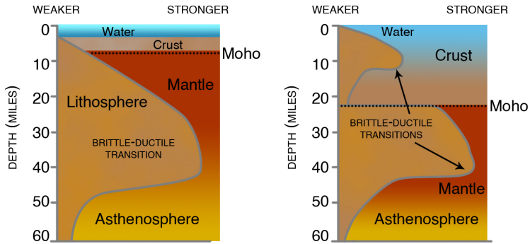
Figure 2-1. Strength of continental lithosphere (crust and upper mantle, above right) compared to oceanic lithosphere (above left). As rocks get buried, they get hotter due to the Earth's geothermal gradient. They also get stronger—down to a point, where temperature takes over, and they abruptly get weaker, at a level called the brittle-ductile transition. The Mohorovičić discontinuity (Moho for short) marks the boundary between the crust, made up of granite and basalt, and the mantle, made up of peridotite. Temperature softens granite at a much shallower depth than peridotite, so that the lower continental crust is a soft, squishy layer between the brittle upper crust and the brittle upper mantle. Earthquakes are limited to the brittle layers of continental crust, and they tend to nucleate where the crust is strongest, just above the brittle-ductile transition to soft, plastic lower crust below. For oceanic lithosphere, the Moho is so shallow that there is no soft layer. The hard lithosphere makes up the tectonic plates. The base of the lithosphere is where peridotite in the mantle becomes soft at high temperature. The soft stuff beneath is the asthenosphere. From Yeats et al. (1997), with permission
