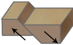
Normal Fault
