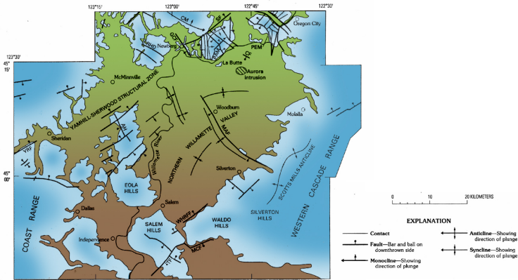
Figure 6-16. Tectonic map of the northern Willamette Valley, showing faults (lines with filled circle toward downthrown side) and folds: .anticlines (arrows face away from thin lines), synclines (arrows face toward thin lines), monoclines (single arrow faces away from thin lines) mapped based on seismic-reflection profiles and exploratory wells drilled in the search for oil and gas. MAF, Mount Angel Fault. Although the Mount Angel Fault later was blamed for the 1993 Scotts Mills Earthquake, it is not clear whether the other faults or any of the folds are active. Portland is just to the north of the figure. From Yeats et al. (1996) and mapping by Ken Werner
