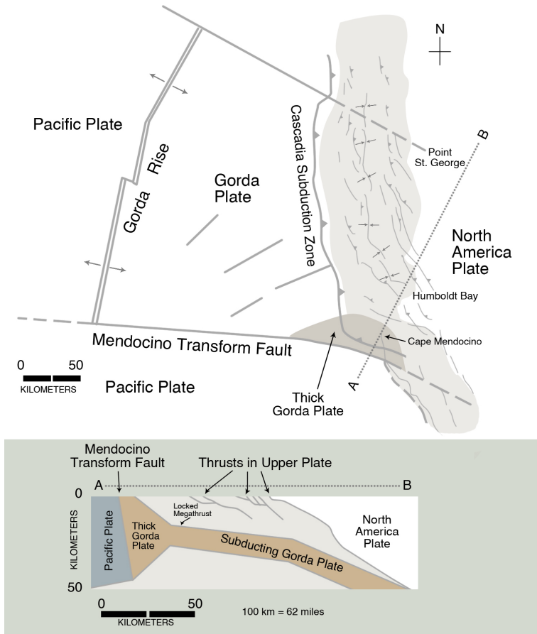
Figure 5-2. The Cascadia Subduction Zone approaches the coastline in northern California, where active folds and thrust faults have been studied by Gary Carver and his associates at Humboldt State University. The subduction zone ends at the Mendocino Transform Fault, which turns southeast to become the San Andreas Fault. The Gorda Plate and spreading center (Gorda Rise) are also shown. The plate is being internally deformed along the Cascadia Subduction Zone and Mendocino Transform Fault.
