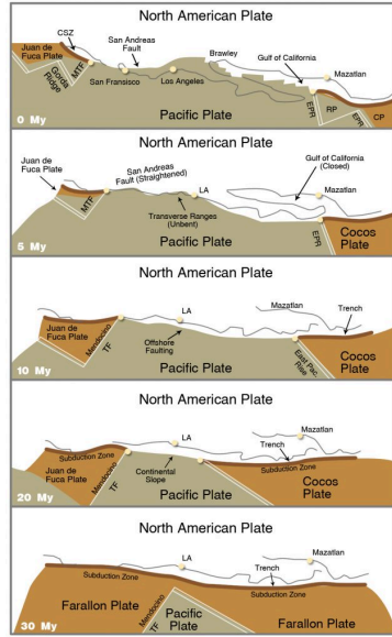
Figure 2-7. At 30 m.y., the oceanic Farallon Plate was subducting under the North America Plate. The double line marks the East Pacific Rise, where the Pacific and Farallon plates were moving apart by sea-floor spreading. The single line at left marks the Mendocino Transform Fault (MTF), which at that time was west of the future location of Los Angeles (LA). The Pacific Plate was moving northwest at the same time that North America was being driven westward by sea-floor spreading on the Mid-Atlantic Ridge. By 20 m.y., the Pacific and North America plates had met at a transform fault at the base of the continental slope.
