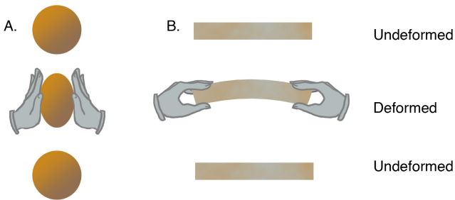
Figure 3-1. Elasticity. (a) An inflated balloon is squeezed between two hands, changing its shape. If the hands are removed, the balloon returns to its earlier shape. (b) A thin board is bent into a curved shape. If the hands bending the board are removed, the board returns to its original shape. The balloon and board are both elastic.
