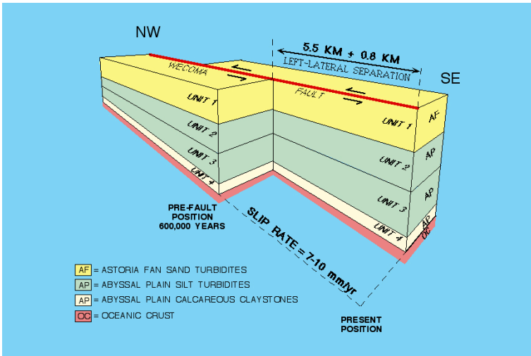
Figure 4-3b. 3D diagram showing how differences in thickness of faulted layers can be matched to give total strike slip on fault. If the age of the layers is known, the rate of slip on the fault may be determined. Based on work by Chris Goldfinger.
