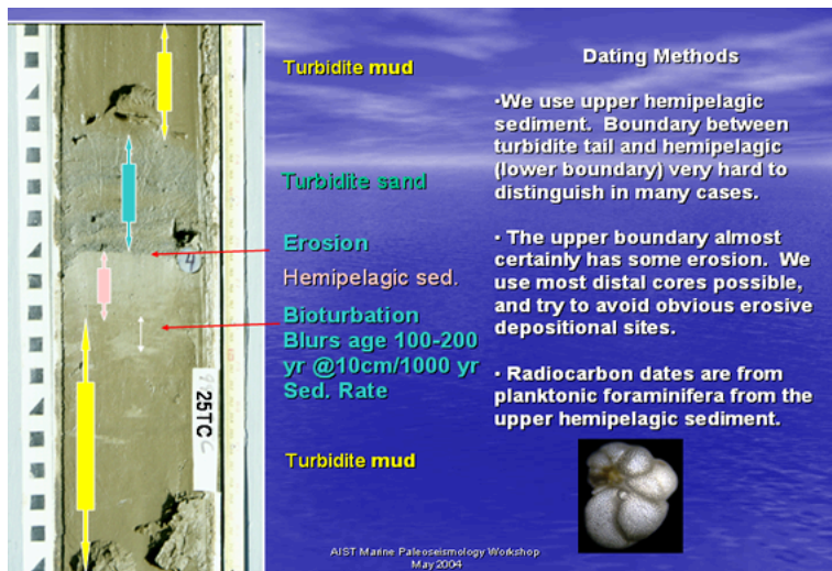
Figure 4-8. Earthquake-generated Cascadia turbidity-current deposit. The cores are dated using microfossils from the fine-grained hemipelagic layer, deposited between successive turbidites. Image courtesy Chris Goldfinger.
