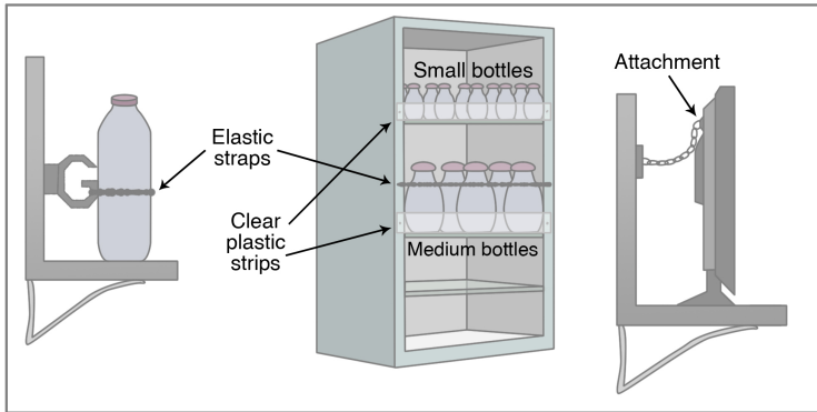
Figure 11-12. Securing items on open shelves: (Left) Attach counter-top items to wall with bungee cord. (Center) Secure small items with a vertical strip and larger items with a strip and bungee cord. (Right) Large items, like a TV set, can be attached to wall with chain.
