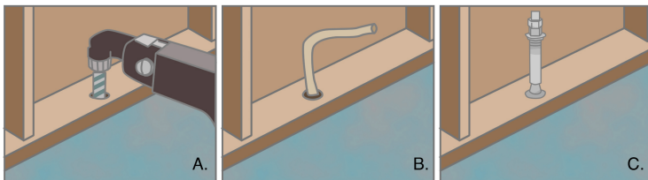
Figure 11-1. Bolt cripple wall (pony wall) to foundation through mudsill, using a sill bolt. (A) Drill hole, using a right-angle drill. (B) Blow powder out of hole, using flexible tubing. (C) Hammer in sill bolt. Tighten nut to expand bolt. From USGS
