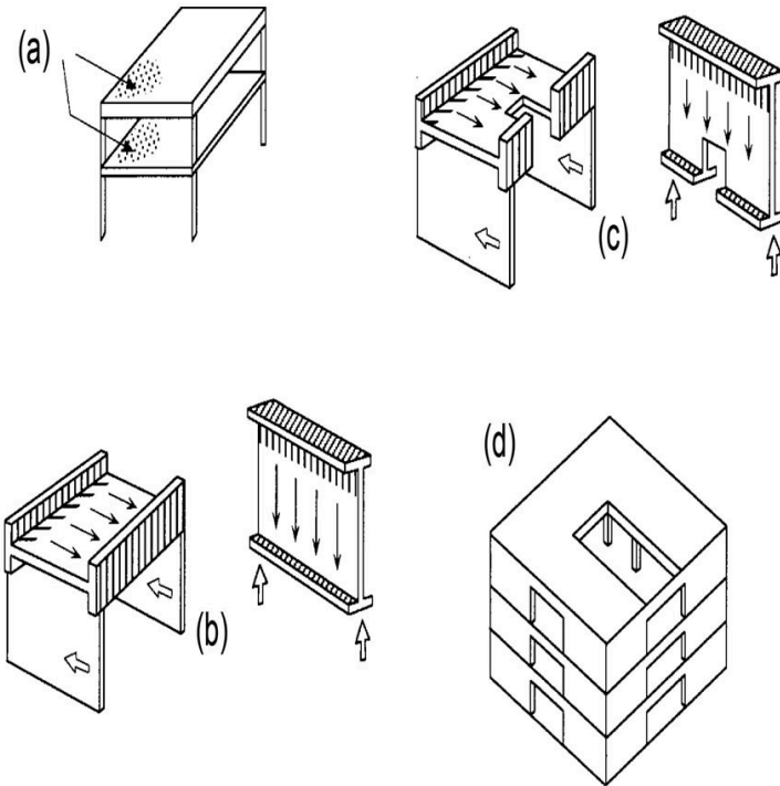
Figure 12-4. (a) A Horizontal diaphragm. Failure typically occurs at connections to vertical columns. (b) Concept of diaphragm as a horizontal I-beam. (c), (d) Holes in beams or diaphragms for elevator shafts, large doors, etc., interrupt continuity and reduce strength. From AIA/ACSA Council on Architectural Research.
