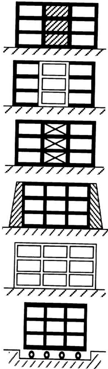
Figure 12-3. Possible retrofit strategies for old buildings. (a)
