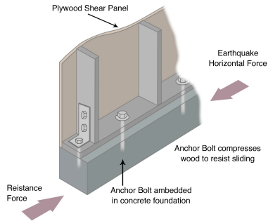
Figure 11-2. Anchor cripple wall to foundation using sill bolts, and to mudsill by hold-down. Cripple wall is further strengthened by plywood shear panel. From Earthquake Engineering Research Institute
