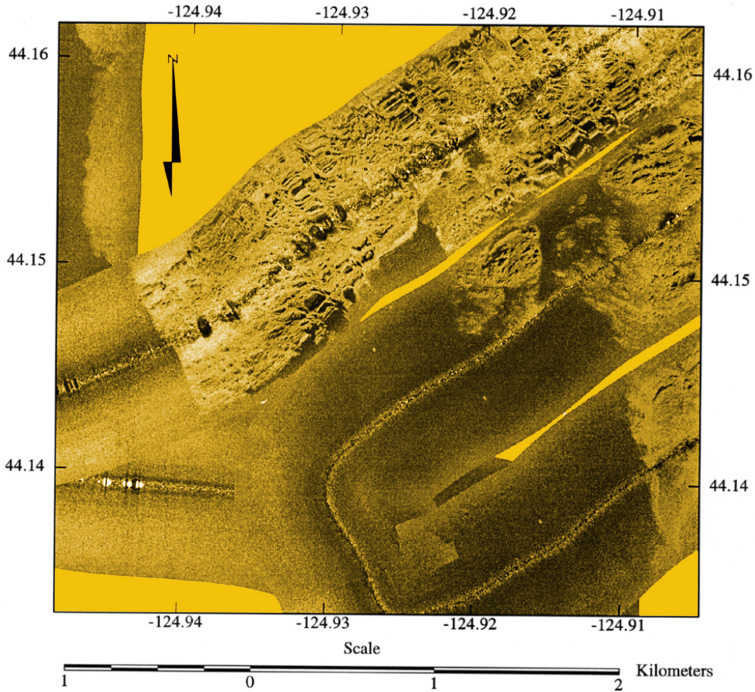
Figure 6-34. The other Oregon coast. Sidescan sonar imagery outlines a shoreline angle developed at the maximum Pleistocene ice advance twenty-one thousand years ago on the west side of Heceta Bank west of Florence, now covered with four hundred feet of sea water. Visible are rocky cliffs (like the present coastline north of Otter Rock) and the mouth of a Pleistocene river. Some of the rocks at the base of the cliffs have been bored in shallow water by marine organisms. The dark gray region in the lower left half of the picture is the former marine erosion platform, now covered with Holocene mud. The Heceta Bank shoreline angle is warped and deformed, evidence of deformation of the Oregon continental shelf.
