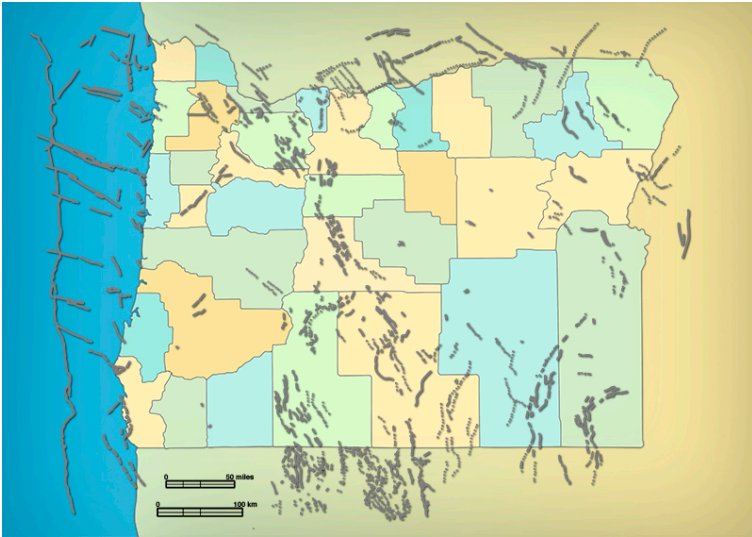
Figure 14-1. Map showing recent faults in Oregon, adjacent states, and the offshore region. Solid lines: faults with demonstrated movement in the past 20,000 years; irregular solid line at left margin marks Cascadia Subduction Zone. Dashed lines: faults with demonstrated movement in past 280,000 years. Dotted lines: faults with demonstrated movement in past 1,800,000 years. Faults shown as dashed or dotted lines could be active, but this has not been demonstrated on geological evidence. From Geomatrix Consultants (1995) and Oregon Department of Geology and Mineral Industries
