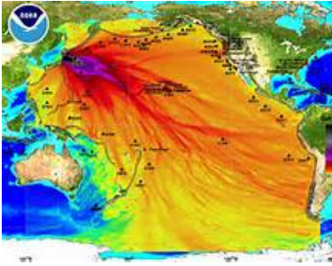
Figure 9-14. Tsunami wave heights from the Tohoku-oki earthquake of March 11, 2011. Darker colors indicate higher wave heights. Note location of DART buoys. Source: NOAA.
