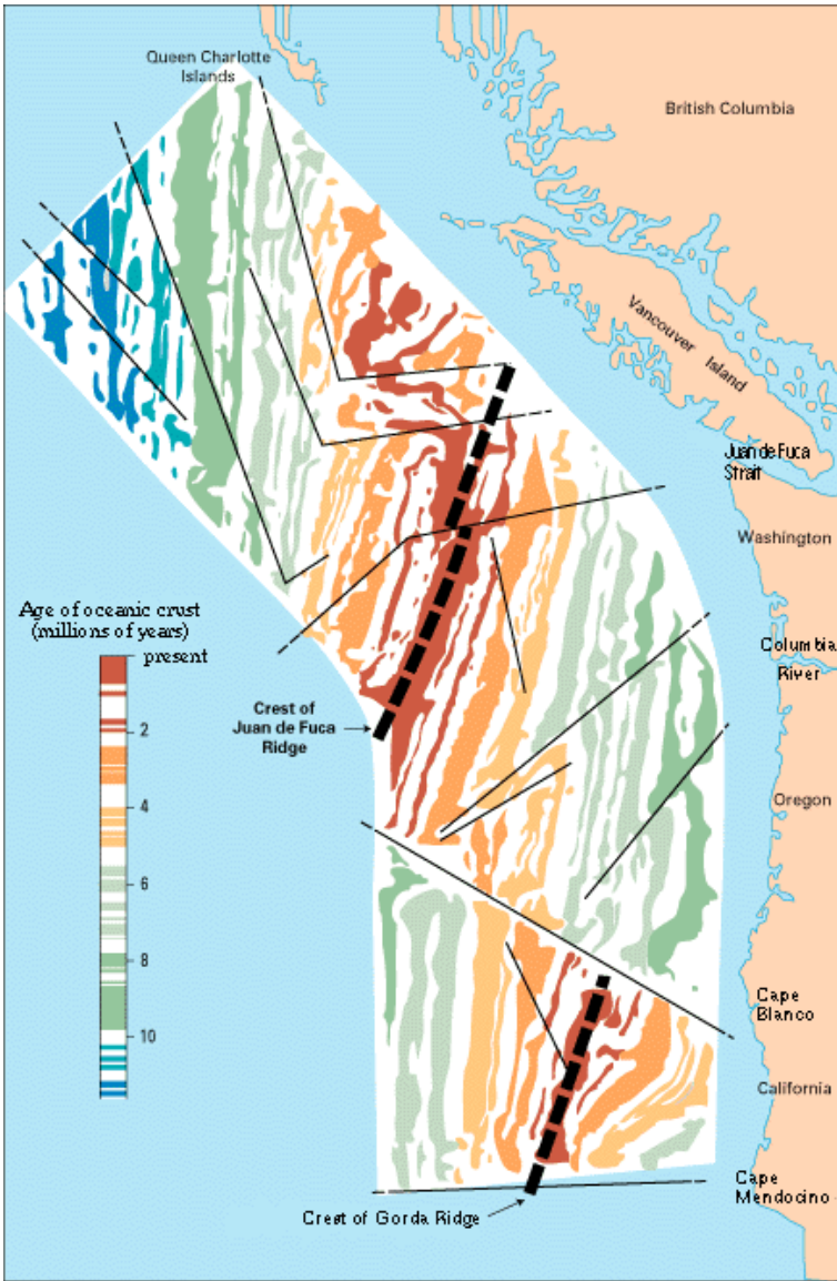
Figure 2-6b. Magnetization map of Cascadia. Colored bands show oceanic crust of normal polarity (magnetic needle points north), and colorless bands show crust of reversed polarity (needle points south). Because we know the age of boundaries of
