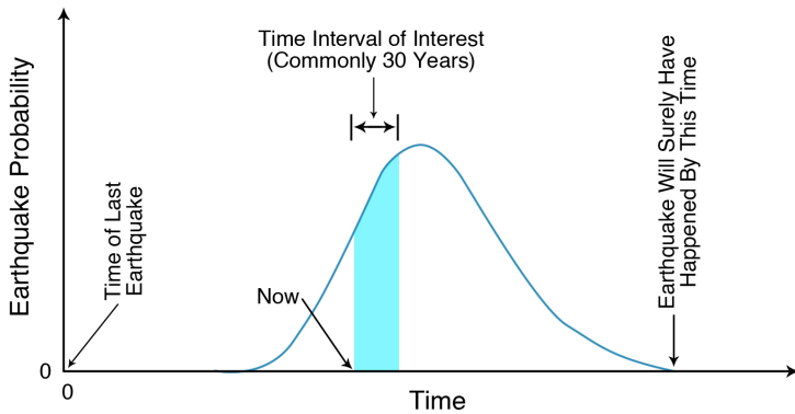
Figure 7-6. The probability for the recurrence of large earthquakes on a given fault or in a given region. Time increases from left to right, and the higher the curve, the greater the likelihood of an earthquake. The previous earthquake happened at time 0. The dark gray band is the time of interest for the probability calculation, commonly thirty years. The left side of the dark band is today. According to this probability, the earthquake will surely have happened by the time the probability curve returns to zero at the right side of the curve.
