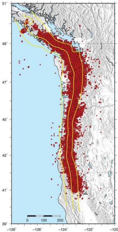
Fig. 4-25. Epicenters of episodic tremor and slip from 2006 to 2009 in Cascadia, from Aaron Wech, University of Washington, and the IRIS (Incorporated Research Institutions for Seismology) Image Gallery. Yellow contours are at 20, 30, and 40 km depth on the subduction zone. West of these epicenters, the Cascadia subduction zone is locked.
