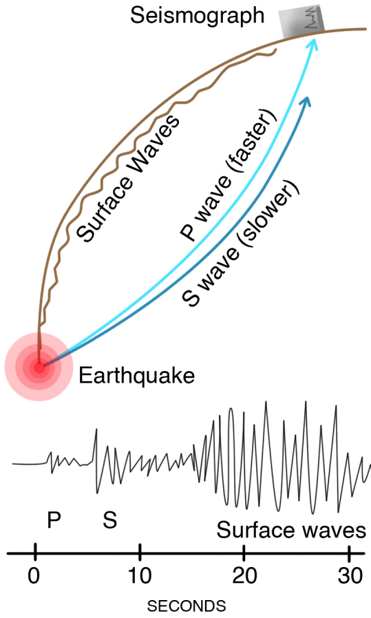
Figure 3-11. An earthquake produces P waves, or compressional waves, that travel faster and reach the seismograph first, and S waves, or shear waves, that are slower. Both are transmitted within the Earth and are called body waves. Even slower are surface waves that run along the surface of the earth and do a lot of the
