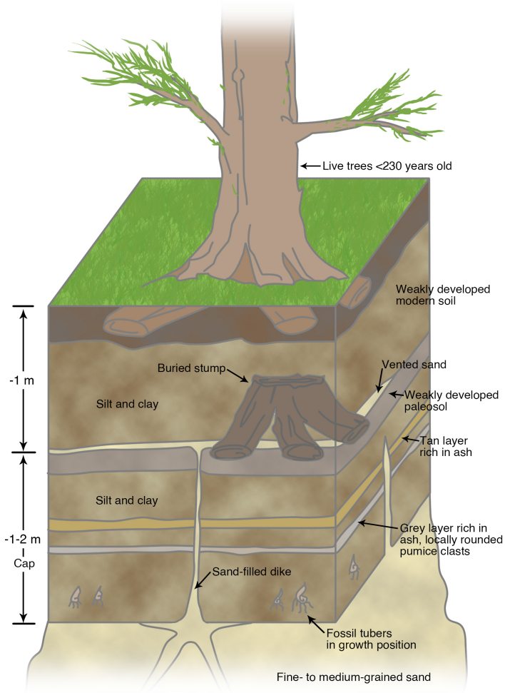
Figure 8-9. Block diagram showing field relations at liquefaction sites on islands in the lower Columbia River. Sand-filled dike cuts through silt and clay with a poorly developed soil at top. Dike connects to thin sand sheet on top of soil that may be remains of sand boil. Tubers have radiocarbon ages of six hundred to one thousand years. Silt and clay on top of sand sheet is younger than dike emplacement; oldest living trees are less than 230 years old. (1 m = just over 3 feet 3 inches). From Steve Obermeier, USGS
