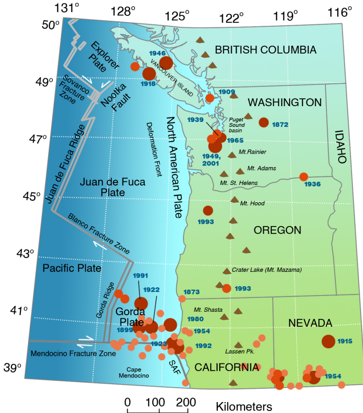
Figure 2-6a. Plate tectonics of the Pacific Northwest. Oceanic crust is formed at the Juan de Fuca Ridge and Gorda Ridge and a ridge west of the Explorer Plate (double lines), adding to the size of the Pacific Plate to the west and the Gorda, Juan de Fuca, and Explorer plates to the east. The plates east of the spreading center are carried beneath North America at the Cascadia Subduction Zone (see Figure 2-5) at the deformation front. Beneath the continent, they give rise to the Cascade volcanoes (shaded triangles). Shaded circles locate larger earthquakes (see also Appendix A). Offshore earthquakes on Blanco Fracture Zone and in and around the Explorer Plate not shown. SAF, San Andreas Fault. Modified from USGS.
