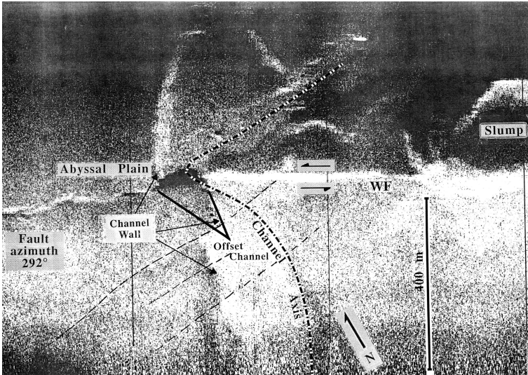
Figure 4-1. Elvis image, marking point of discovery of the Wecoma Fault, which offsets a deep-sea channel about one hundred meters (more than three hundred feet). Slip rate on this left-lateral strike-slip fault is about one inch every four years. Image acquired by SeaMarc 1A side-scan sonar, with sound coming from bottom of image. (Elvis's head and upper body, holding a guitar, are at top of image.) Image courtesy of Chris Goldfinger, College of Earth, Ocean, and Atmospheric Sciences, Oregon State University.
