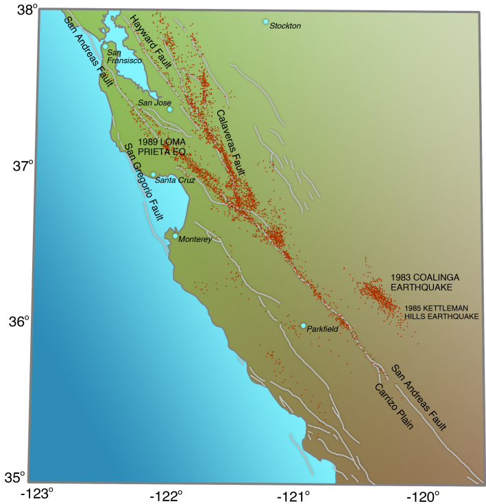
Figure 7-5. Seismicity of central California, 1980-1986, to compare the seismicity of that part of the San Andreas Fault that ruptured in 1857 (southeast, or lower right corner), which does not image the fault at all, to the seismicity of that part of the San Andreas Fault that ruptures frequently, as at Parkfield, or creeps accompanied by very small earthquakes, which images the fault very well. That part of the fault in the northwest, or upper left corner of the map, ruptured in 1906, but is not well imaged by microearthquakes. From David Oppenheimer, USGS
