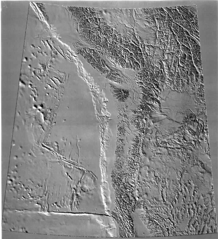
Figure 4-5. Computer-generated map (Digital Elevation Model or DEM) of Pacific Northwest, both on land and offshore. The continental slope is the boundary between the continental North American Plate and oceanic Juan de Fuca and Gorda plates, which is the Cascadia Subduction Zone. North of Vancouver Island, the boundary is the Queen Charlotte strike-slip fault. The Gorda and Juan de Fuca ridges and Blanco Fracture Zone are visible on the deep ocean floor. Note the Mendocino Fracture Zone at the southern end of the DEM, which is the boundary with the Pacific Plate to south.
