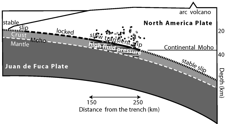
Fig. 4-26. Cross section through Cascadia subduction zone showing subdivision into a zone of stable sliding closest to the trench, the locked zone subject to great earthquakes, the zone of episodic tremor and slip, possibly related to high fluid pressure (epicenters in Fig. 4-25), and deep zone of stable sliding extending beneath the volcanic arc. From Gomberg et al. (2010).
