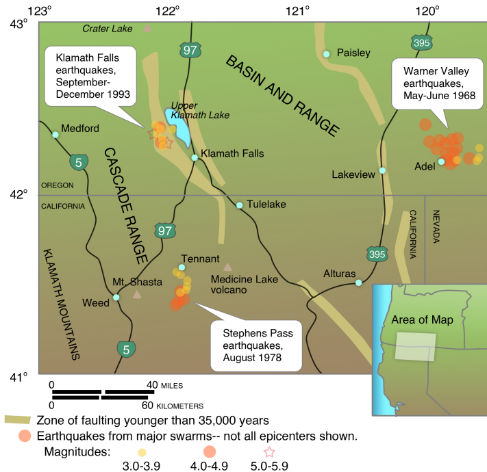
Figure 6-29. Map showing locations of recent earthquake swarms in southern Oregon and northern California, including the Warner Valley, Oregon, earthquakes of 1968. From USGS.
