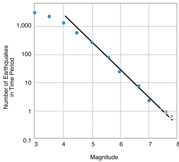
Figure 7-3. Illustration of the Gutenberg-Richter (G-R) relationship for thirty years of seismicity data for the Imperial Valley of southern California. Shown are the number of earthquakes of a given magnitude for the time period. Note that both scales are logarithmic, that is, each unit is ten times larger than the preceding one, as earlier discussed for magnitude. For this reason, the straight line may be somewhat misleading. The drop-off in seismicity for lower magnitudes is generally related to the sensitivity of the seismic network; it does not record all the smaller events. Projecting the straight line downward, G-R predicts 0.4 earthquakes of M 8 in the thirty-year time period, or one M 8 earthquake every seventy-five years. This prediction is questionable, as is the timing of still larger earthquakes. From C. R. Allen, Caltech, in Yeats et al. (1997)
