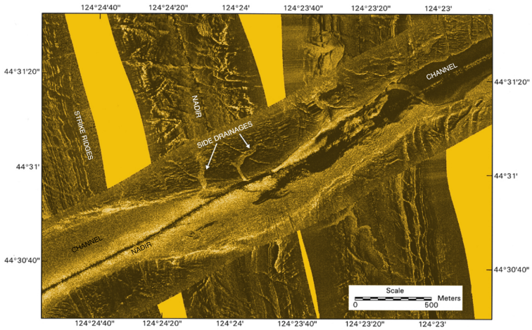
Figure 6-35. Sidescan sonar image of a river channel crossing Stonewall Bank, southwest of Newport, now covered with two hundred feet of sea water. The channel, marking the seaward continuation of the Yaquina River, is now tilted eastward, evidence of deformation of the Oregon continental shelf in the last twelve thousand years. Image courtesy of Chris Goldfinger, College of Oceanic and Atmospheric Sciences, Oregon State University; see also Yeats et al. (1998)
