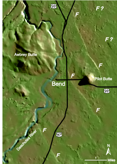
Figure 6-30. Computer-generated topographic map of Bend, Oregon, region showing young faults (linear features marked F). Image is illuminated by a light source from northeast that is 15 degrees above the horizon; accordingly, fault scarps that face northeast are brightly lit, whereas fault scarps facing southwest (such as the lineation marked F? north of Pilot Butte) are in shadow. These faults cut volcanic materials and sediments as young as late Pleistocene, but are not known to cut Holocene deposits. The prominence of these faults may be due to the greater consolidation of the deposits cut by them rather than their Holocene age. The fault scarp in
