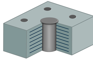
Figure 12-9. Base-isolation bearing. Alternating laminations of rubber and steel with a lead plug in the middle. From AIA/ACSA Council on Architectural Research
