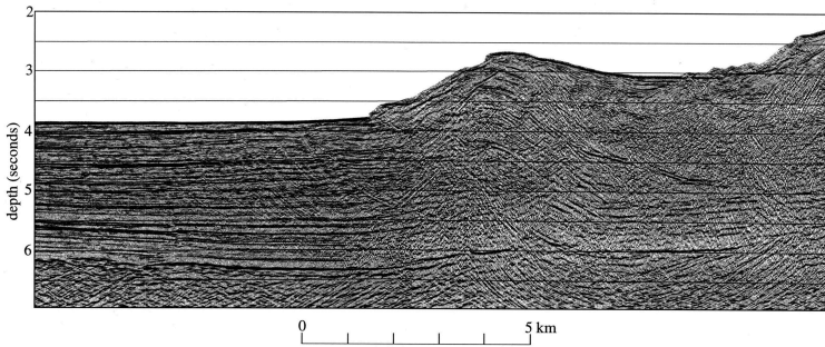
Figure 4-2. Seismic-reflection profile of the Cascadia Subduction Zone off central Oregon. West is to the left. Signals from a ship were bounced off the sea floor and off more deeply buried sediment layers, then echoed back to the ship, allowing a profile to be made that shows the geology beneath the sea floor. The flat sea floor on the left is the sediment-covered abyssal plain of the Juan de Fuca Plate. The Cascadia Subduction Zone has thrust highly deformed rocks of the North America Plate over the flat Juan de Fuca Plate. The fault slopes gently to the east. Sediment layers at the left are being forced under the edge of the continent and, in addition, dragged up against the edge of the continent as an accretionary wedge. Profile acquired in 1989 by Digicon for the National Science Foundation. Image courtesy of LaVerne D. Kulm and Chris Goldfinger, College of Earth, Ocean, and Atmospheric Sciences, Oregon State University.
