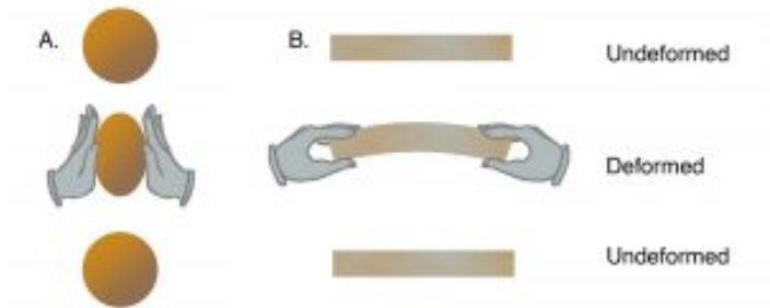
Figure 3-1. Elasticity. (a) An inflated balloon is squeezed between two hands, changing its shape. If the hands are removed, the balloon returns to its earlier shape. (b) A thin board is bent into a curved shape. If the hands bending the board are removed, the board returns to its original shape. The balloon and board are both elastic.
