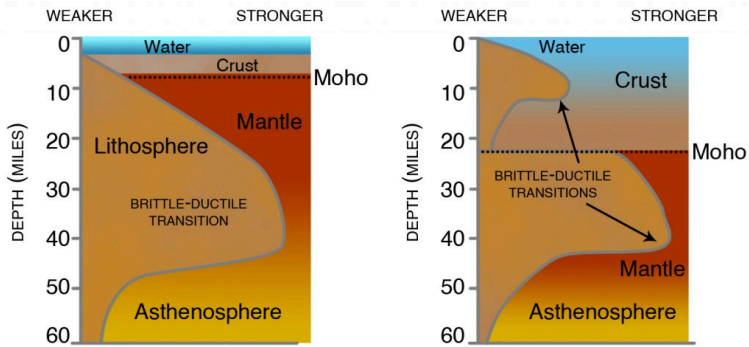
Figure 2-1. Strength of continental lithosphere (crust and upper mantle, above right) compared to oceanic lithosphere (above left). As rocks get buried, they get hotter due to the Earth's geothermal gradient. They also get stronger—down to a point, where temperature takes over, and they abruptly get weaker, at a level called the brittle-ductile transition. The Mohorovičić discontinuity (Moho for short) marks the boundary between the crust, made up of granite and basalt, and the mantle, made up of peridotite. Temperature softens granite at a much shallower depth than peridotite, so that the lower continental crust is a soft, squishy layer between the brittle upper crust and the brittle upper mantle. Earthquakes are limited to the brittle layers of continental crust, and they tend to nucleate where the crust is strongest, just above the brittle-ductile transition to soft, plastic lower crust. For oceanic lithosphere, the Moho is so shallow that there is no soft layer. The hard lithosphere makes up the tectonic plates. The base of the lithosphere is where peridotite in the mantle becomes soft at high temperature. The soft stuff beneath is the asthenosphere. From Yeats et al. (1997), with permission
