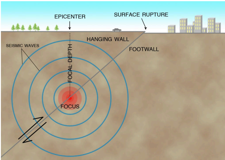
Figure 3-4. A cross section of the Earth's crust.
