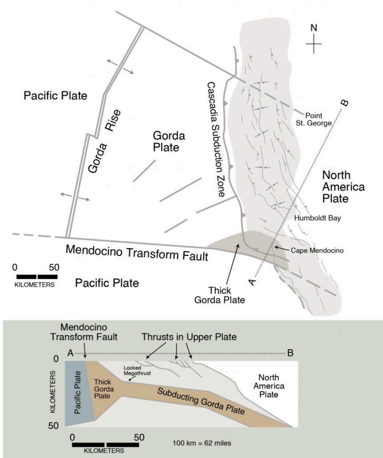
Figure 5-2. The Cascadia Subduction Zone approaches the coastline in northern California, where active folds and thrust faults have been studied by Gary Carver and his associates at Humboldt State University. The subduction zone ends at the Mendocino Transform Fault, which turns southeast to become the San Andreas Fault. The Gorda Plate and spreading center (Gorda Rise) are also shown. The plate is being internally deformed along the Cascadia Subduction Zone and Mendocino Transform Fault.
