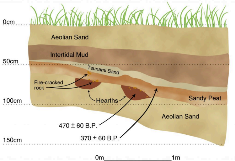
Figure 4-20. Cross section of buried Native American campsite (hearths, fire-cracked rock) overlain by a soil zone submerged by the A.D. 1700 Cascadia Subduction Zone earthquake and covered by a tsunami deposit. From Minor and Grant (1996); drawing courtesy of Rick Minor, Heritage Research Associates, Eugene, Oregon.
