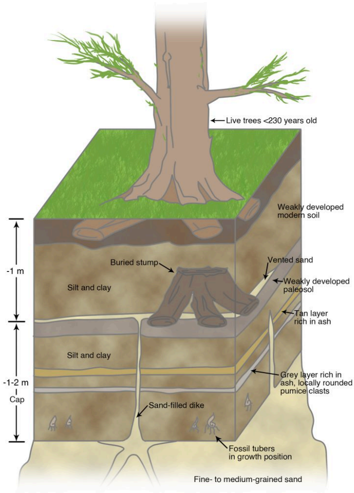
Figure 8-9. Block diagram showing field relations at liquefaction sites on islands in the lower Columbia River. Sand-filled dike cuts through silt and clay with a poorly developed soil at top. Dike connects to thin sand sheet on top of soil that may be remains of sand boil. Tubers have radiocarbon ages of six hundred to one thousand years. Silt and clay on top of sand sheet is younger than dike emplacement; oldest living trees are less than 230 years old. (1 m = just over 3 feet 3 inches). From Steve Obermeier, USGS
