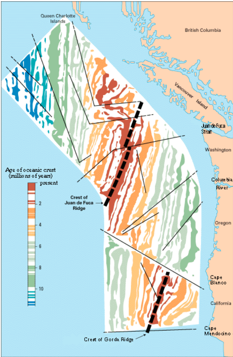
Figure 2-6b. Magnetization map of Cascadia. Colored bands show oceanic crust of normal polarity (magnetic needle points north), and colorless bands show crust of reversed polarity (needle points south). Because we know the age of boundaries of
